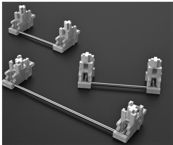
Satellite Axis /Balancing Axle
